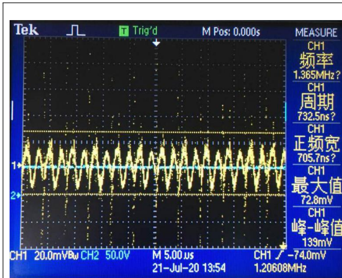
Noise (VIN = 42V, IO = 2.5A, 5 ~ 20MHz bandwidth)
