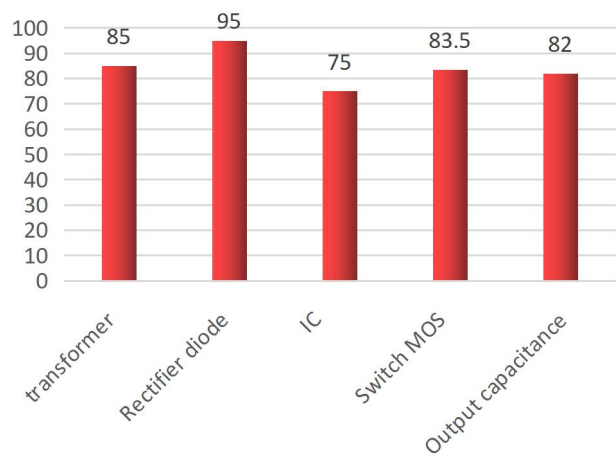
Efficiency ( V_{out} = 5\text{ V} )
