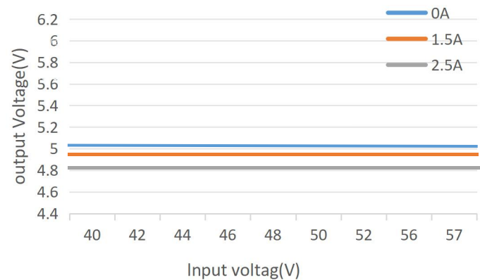
Input voltage & output voltage
