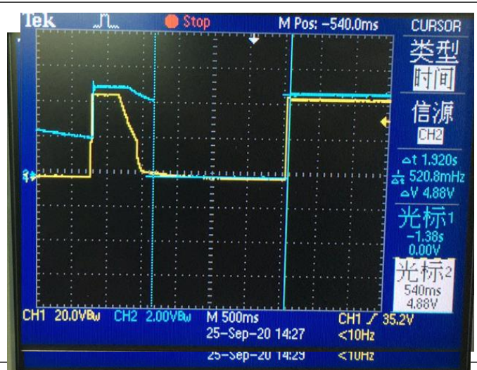
Output response & load (5V / 2.5A)
