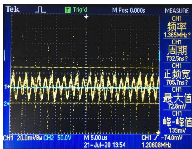
Noise (VIN = 37V, IO = 2A, 5 ~ 20MHz bandwidth)
