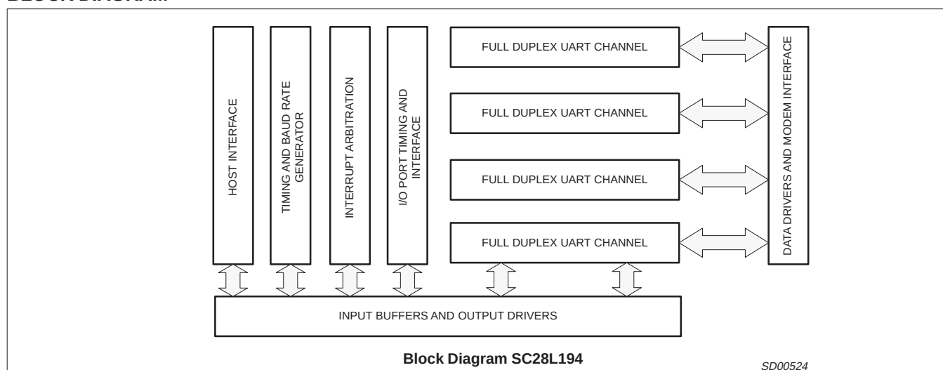
Figure 2. Block Diagram
