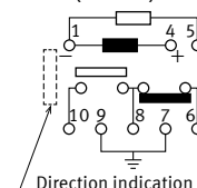
2 coil latching (Reset)
