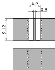
Calibration board
