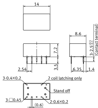
External dimensions
