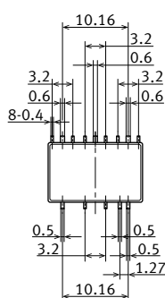
External dimensions
