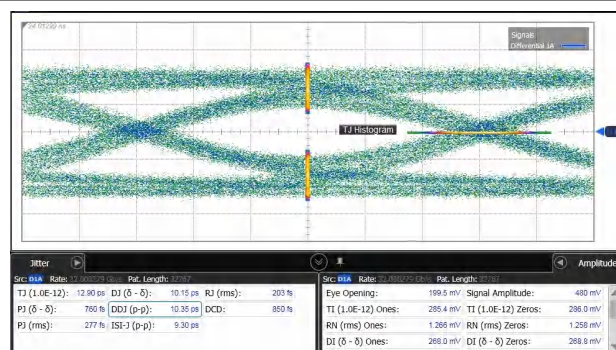
图 6-5. Through Calibration Trace (6.5 dB Loss)
