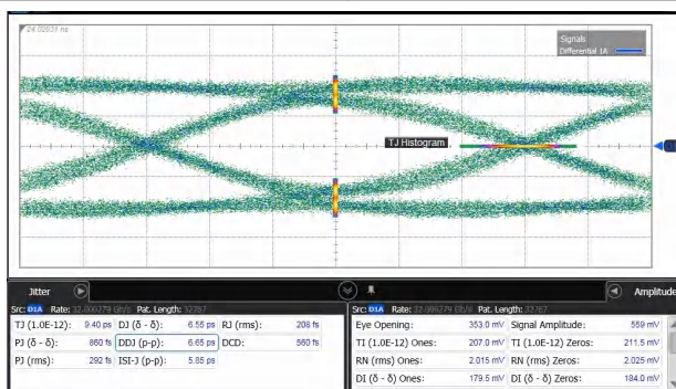
图 6-6. Through SN75LVPE5421 (6.5 dB loss and DUT EQ=0)
