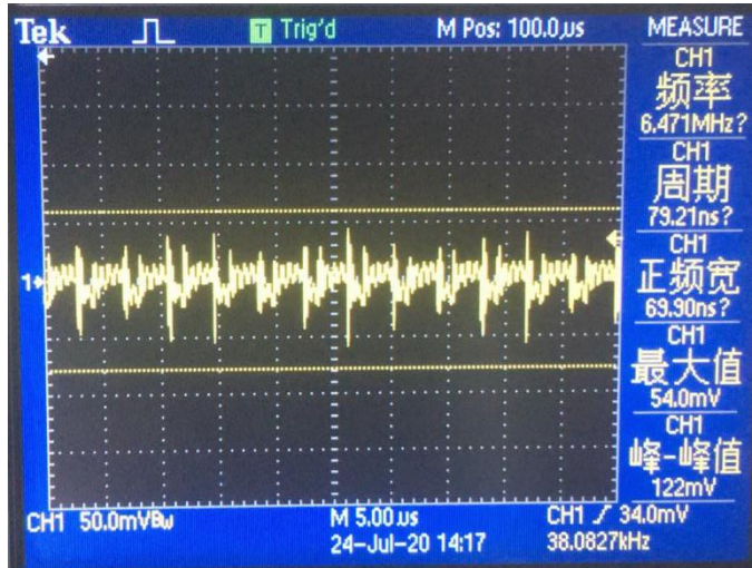
Noise ( V_{IN} = 42V , I_O = 2A , 5 ~ 20MHz bandwidth)
