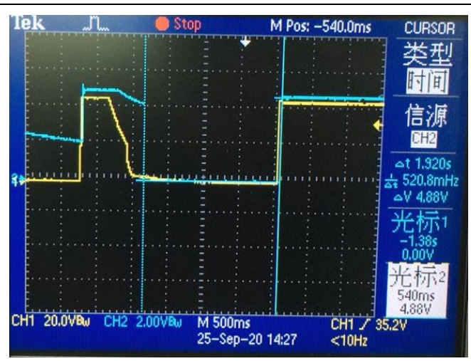
Output response & load (3.3V / 2 A)
