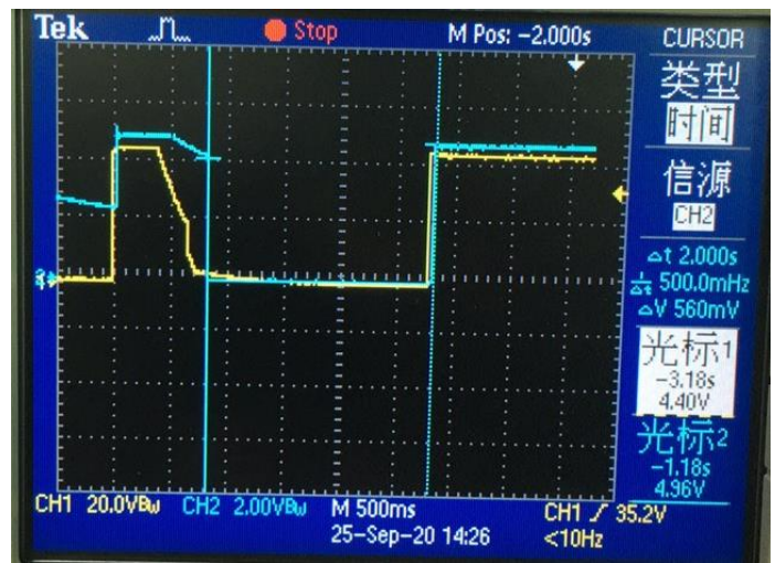
Output response & load (3.3V / 1.5A)
